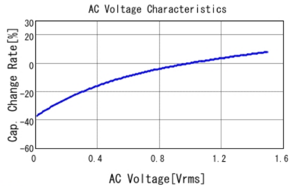
■ GCJ31CR71C106KA15 C-AC Voltage capchange, DCOV, 25.0d
