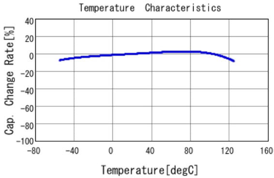
■ GCJ31CR71C106KA15 C-Temp. capchange, DC0.0V, AC1.0Vrm
