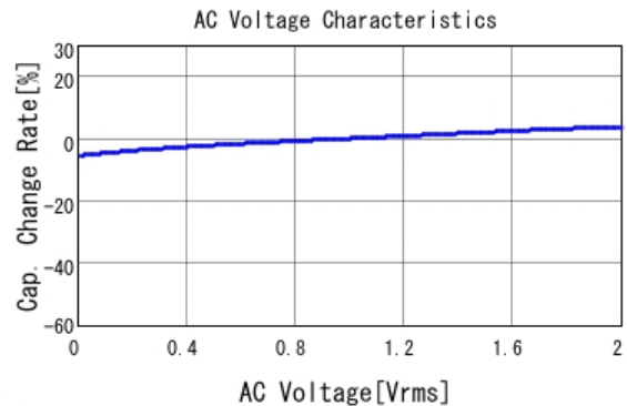
■ GCJ31CR71E475KA12 C-AC Voltage capchange, DC0V, 25.0d
