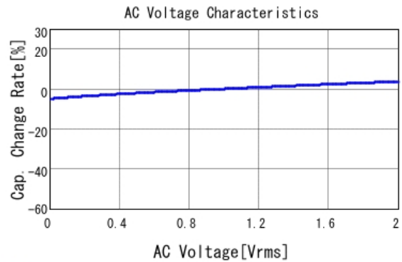
■ GCJ31CR71H225KA12 C-AC Voltage capchange, DC0V, 25.0d
