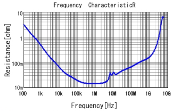
■ GCJ31CR71H225KA12 R DC0V, 25degC
