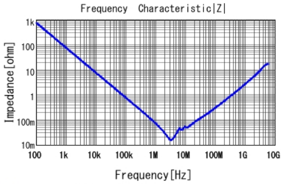
■ GCJ31CR71H225KA12 |Z| DC0V, 25degC
