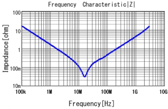
■ GCJ31CR72E104KXJ3 |Z| DC0V, 25degC
