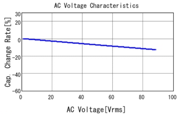
■ GCJ31CR72E104KXJ3 C-AC Voltage capchange, DC0V, 25.0d
