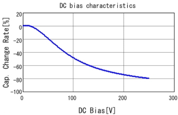
■ GCJ31CR72E104KXJ3 C-DC bias capchange, 25.0degC, AC1V
