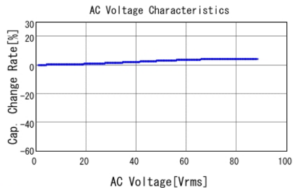
■ GCJ31CR72E473KXJ3 C-AC Voltage capchange, DC0V, 25.0d
