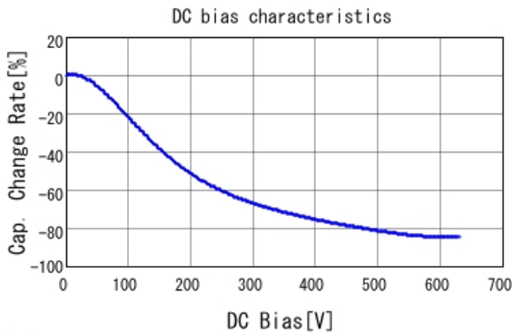
■ GCJ31CR72J223KXJ3 C-DC bias capchange, 25.0degC, AC1V
