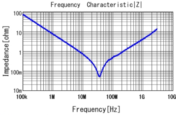
■ GCJ31CR72J223KXJ3 |Z| DC0V, 25degC
