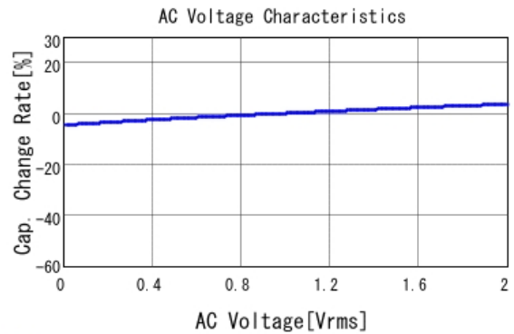
■ GCJ31MR71E105KA01 C-AC Voltage capchange, DC0V, 25.0d
