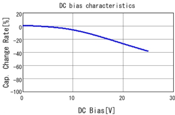
■ GCJ31MR71E105KA01 C-DC bias capchange, 25.0degC, AC1.
