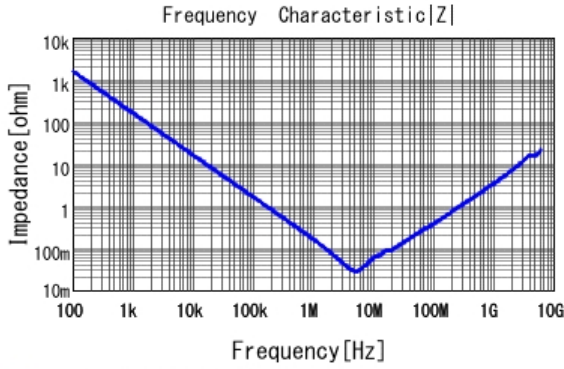
■ GCJ31MR71E105KA01 |Z| DC0V, 25degC
