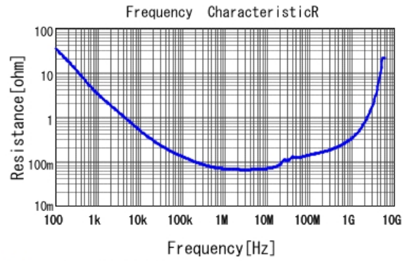
■ GCJ31MR72A224KA01 R DC0V, 25degC
