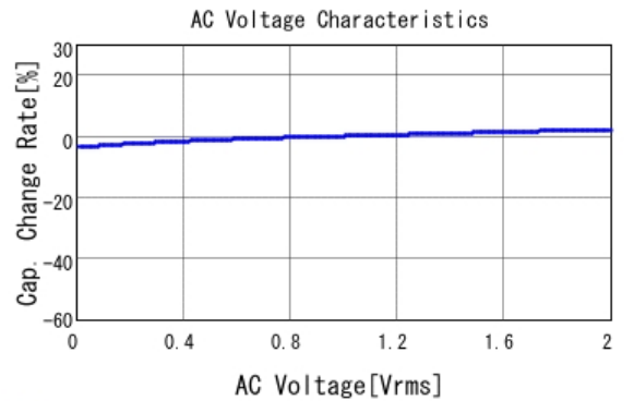
■ GCJ31MR72A224KA01 C-AC Voltage capchange, DC0V, 25.0d
