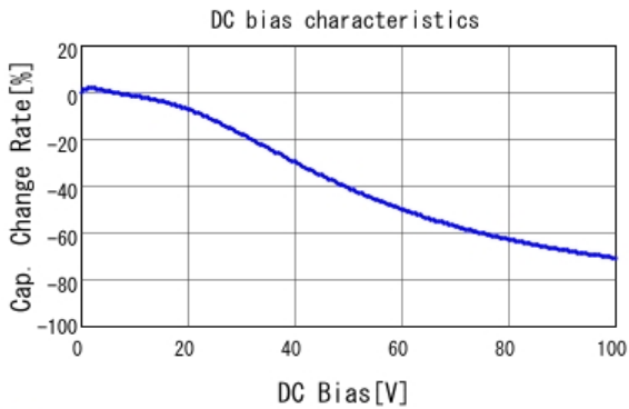
■ GCJ31MR72A224KA01 C-DC bias capchange, 25.0degC, AC1.
