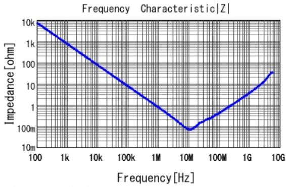
■ GCJ31MR72A224KA01 |Z| DC0V, 25degC
