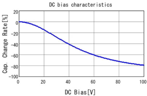
■ GCJ32DR72A225KA01 C-DC bias capchange, 25.0degC, AC1.
