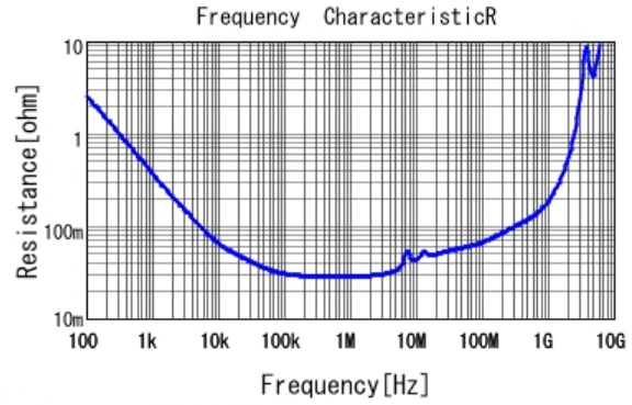
■ GCJ32DR72A225KA01 R DC0V, 25degC
