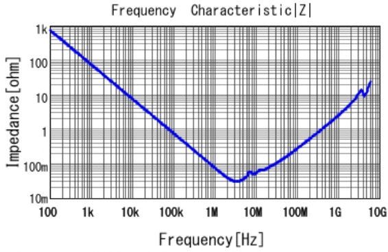
■ GCJ32DR72A225KA01 |Z| DC0V, 25degC
