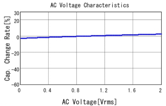
■ GCJ32DR72A225KA01 C-AC Voltage capchange, DC0V, 25.0d
