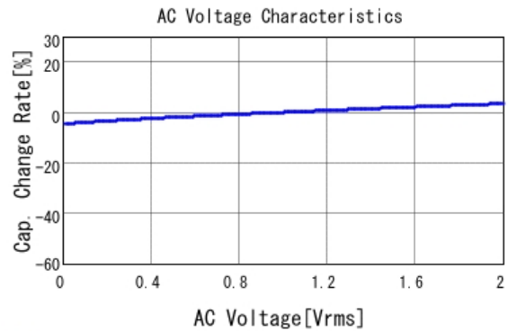
■ GCJ32EL81E475KA01 C-AC Voltage capchange, DC0V, 25.0d
