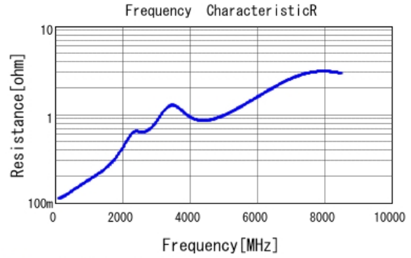
■ GCM0335C1E101JA16 R DCOV, 25degC
