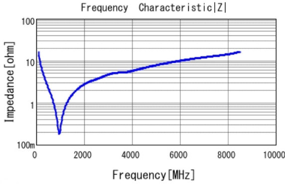
■ GCM0335C1E101JA16 |Z| DCOV, 25degC
