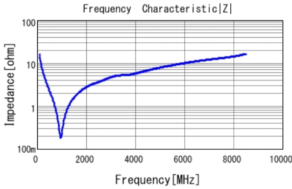
■ GCM0335C1H101JA16 |Z| DCOV, 25degC
