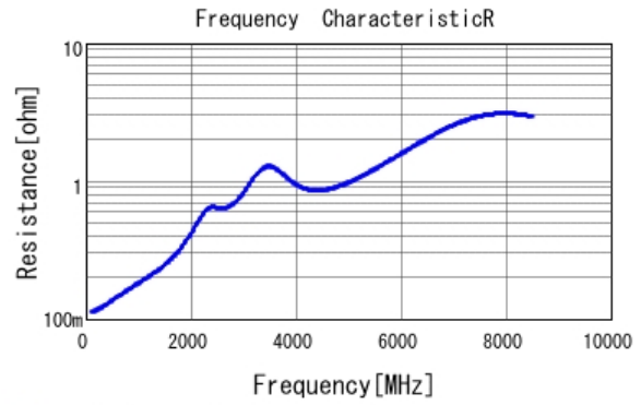
■ GCM0335C1H101JA16 R DCOV, 25degC
