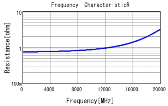
■ GCM0335C1H1R0CA16 R DCOV, 25degC
