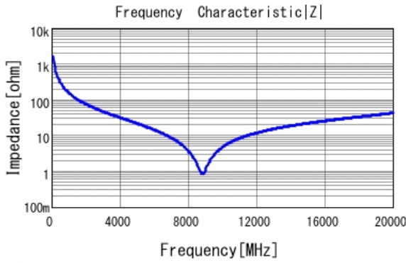
■ GCM0335C1H1R0CA16 |Z| DCOV, 25degC
