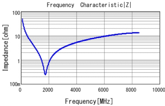
■ GCM0335C1H330JA16 |Z| DCOV, 25degC
