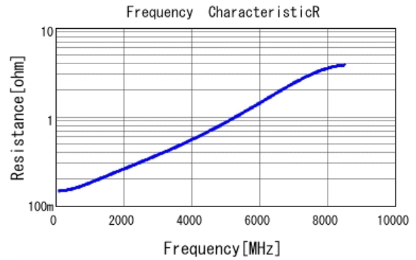
■ GCM0335C1H330JA16 R DCOV, 25degC
