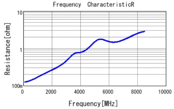
■ GCM0335C1H470JA16 R DCOV, 25degC
