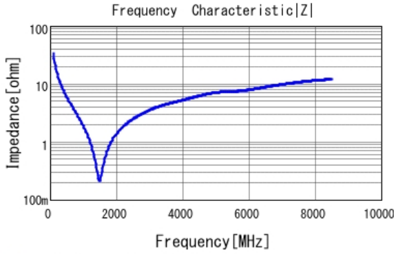
■ GCM0335C1H470JA16 |Z| DCOV, 25degC
