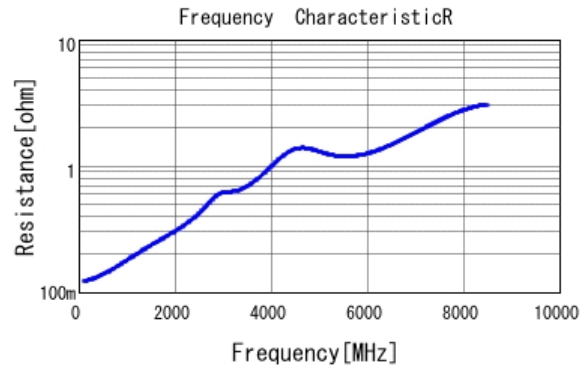
■ GCM0335C1H680JA16 R DCOV, 25degC
