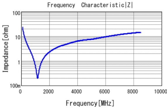
■ GCM0335C1H680JA16 |Z| DCOV, 25degC
