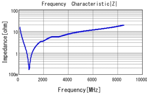
■ GCM1555C1H101JA16 |Z| DCOV, 25degC
