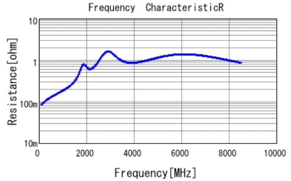
■ GCM1555C1H101JA16 R DCOV, 25degC
