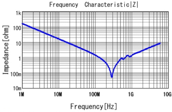
GCM1555C1H102GA16 |Z| DCOV, 25degC
