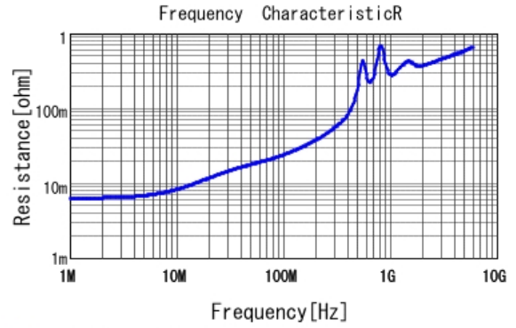
GCM1555C1H102GA16 R DCOV, 25degC
