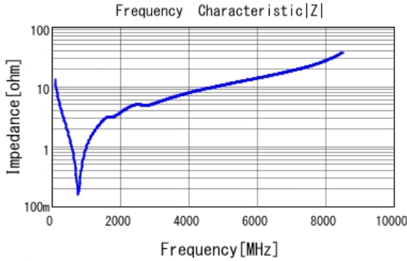
■ GCM1555C1H121JA16 |Z| DCOV, 25degC
