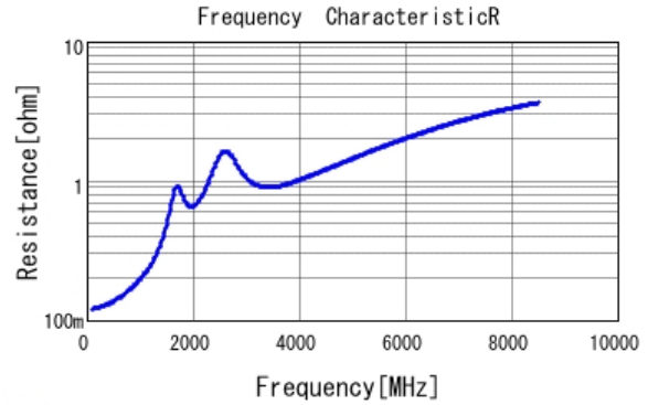
■ GCM1555C1H121JA16 R DCOV, 25degC
