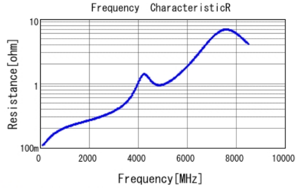
■ GCM1555C1H180JA16 R DCOV, 25degC
