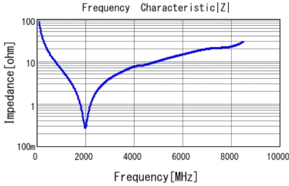
■ GCM1555C1H180JA16 |Z| DCOV, 25degC
