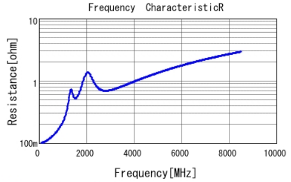
■ GCM1555C1H181JA16 R DCOV, 25degC
