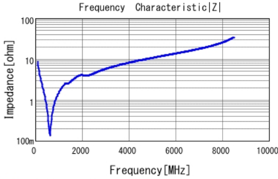
■ GCM1555C1H181JA16 |Z| DCOV, 25degC
