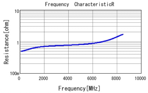
■ GCM1555C1H1R0CA16 R DCOV, 25degC
