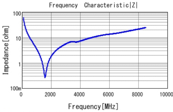
■ GCM1555C1H270JA16 |Z| DCOV, 25degC
