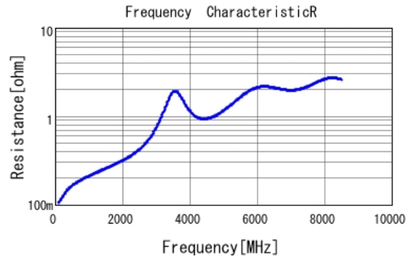
■ GCM1555C1H270JA16 R DCOV, 25degC
