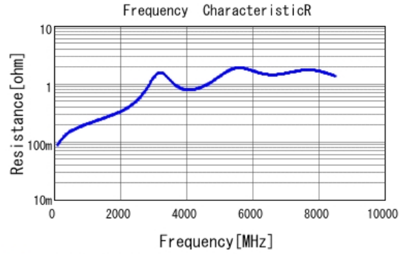
■ GCM1555C1H330JA16 R DCOV, 25degC
