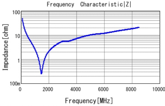
■ GCM1555C1H330JA16 |Z| DCOV, 25degC
