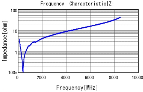
■ GCM1555C1H391JA16 |Z| DCOV, 25degC
