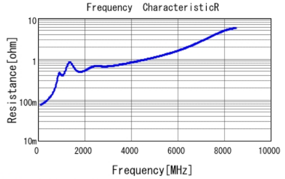
■ GCM1555C1H391JA16 R DCOV, 25degC
