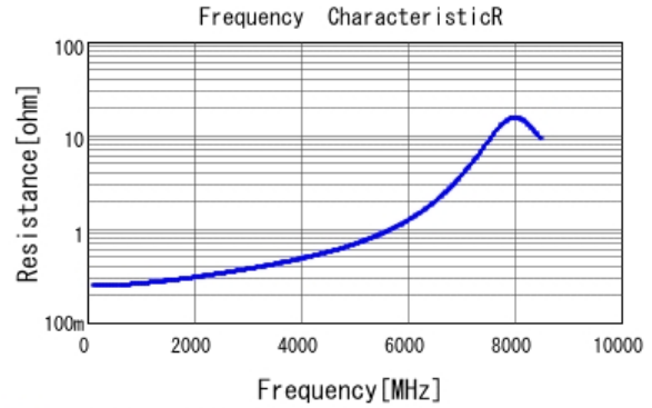
■ GCM1555C1H4R7BA16 R DC0V, 25degC
