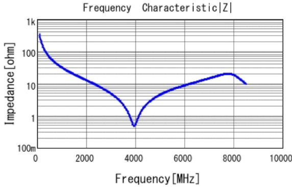
■ GCM1555C1H4R7BA16 |Z| DC0V, 25degC
