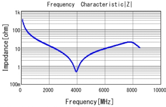
■ GCM1555C1H4R7CA16 |Z| DCOV, 25degC
