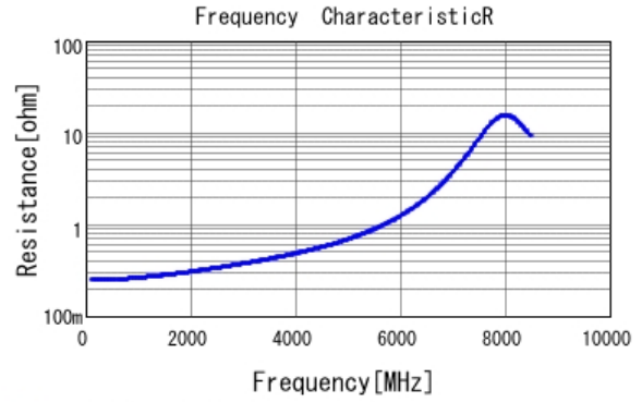
■ GCM1555C1H4R7CA16 R DCOV, 25degC
