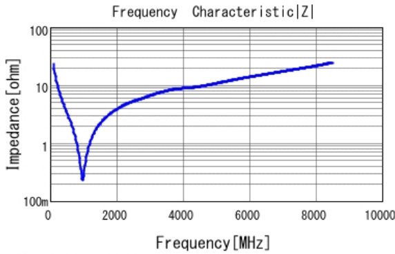
■ GCM1555C1H680JA16 |Z| DCOV, 25degC
