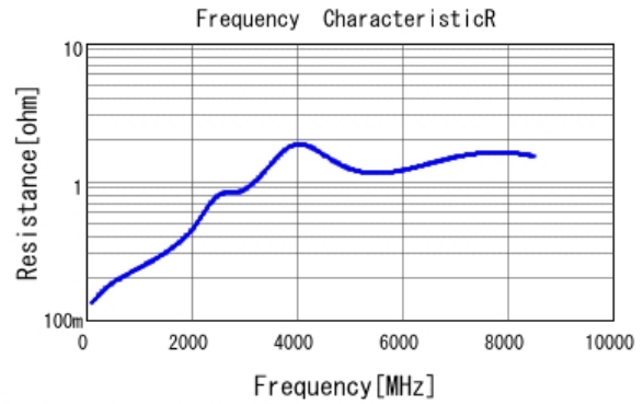
■ GCM1555C1H680JA16 R DCOV, 25degC
