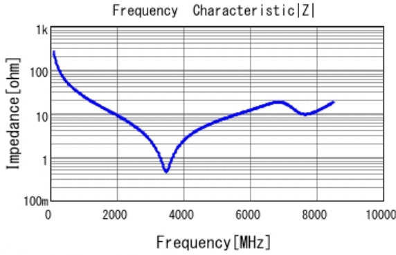
■ GCM1555C1H6R0DA16 |Z| DCOV, 25degC
