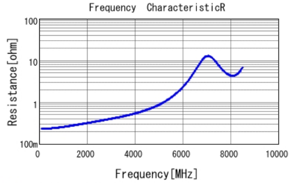
■ GCM1555C1H6R0DA16 R DCOV, 25degC
