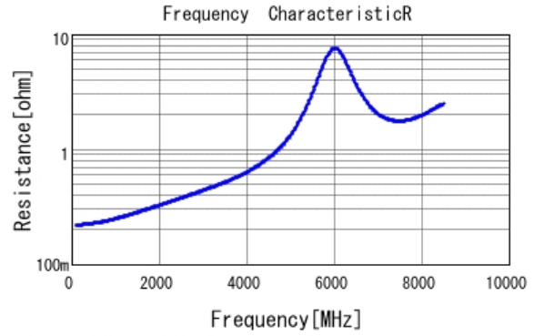
■ GCM1555C1H8R2BA16 R DCOV, 25degC
