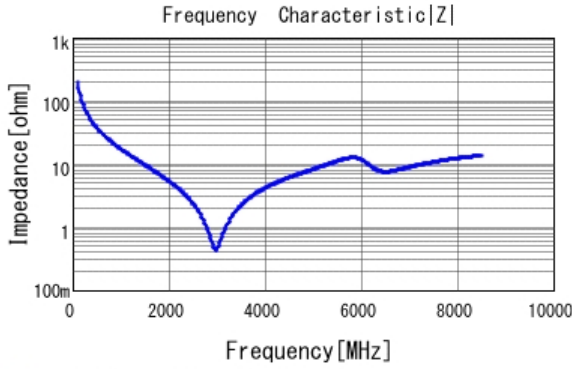
■ GCM1555C1H8R2BA16 |Z| DCOV, 25degC
