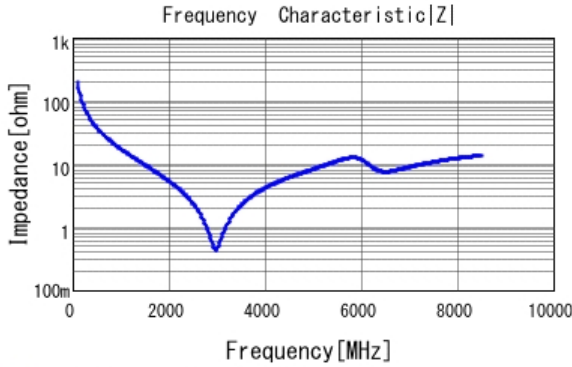
■ GCM1555C1H8R2CA16 |Z| DCOV, 25degC
