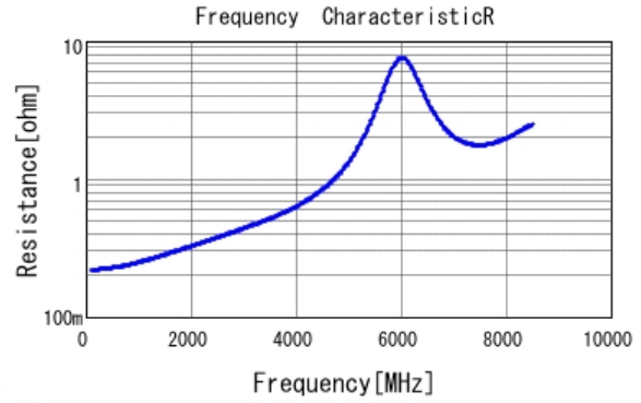
■ GCM1555C1H8R2DA16 R DCOV, 25degC
