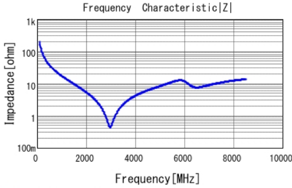
■ GCM1555C1H8R2DA16 |Z| DCOV, 25degC
