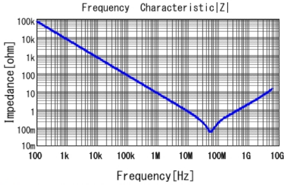
GCM155R71E223KA55 |Z| DCOV, 25degC
