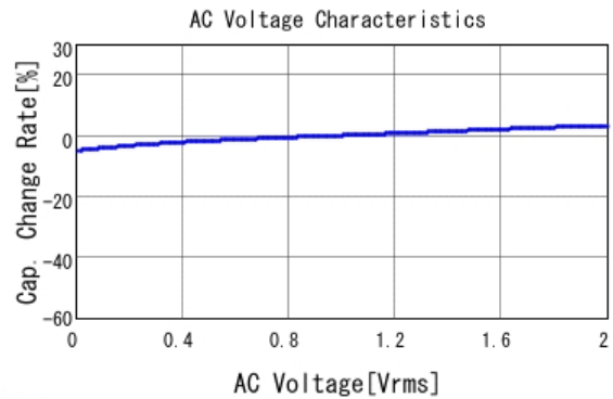
■ GCM155R71E473KA55 C-AC Voltage capchange, DCOV, 25.0d
