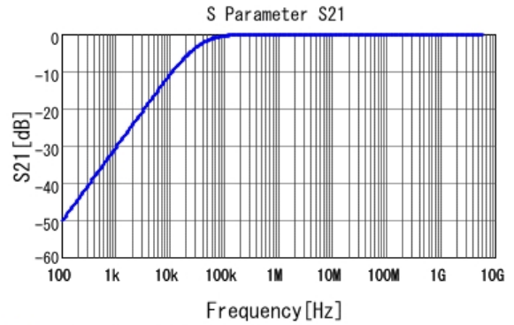
■ GCM155R71E473KA55 S21 DC0V, 25degC
