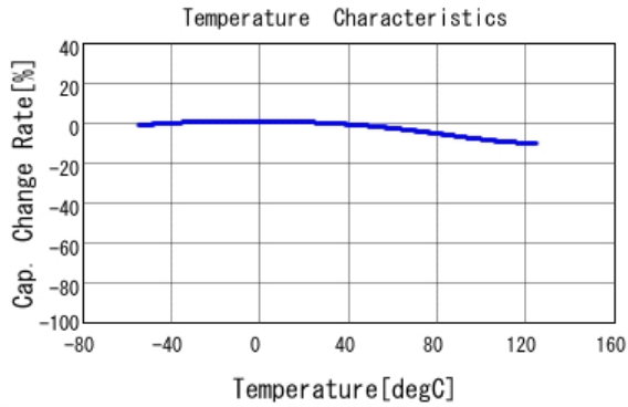
■ GCM155R71E473KA55 C-Temp. capchange, DC0.0V, AC1.0V rm
