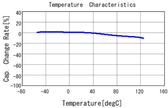
■ GCM155R71H333KE02 C-Temp. capchange, DC0.0V, AC1.0V rm
