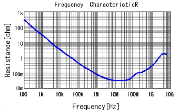
GCM155R71H333KE02 R DCOV, 25degC
