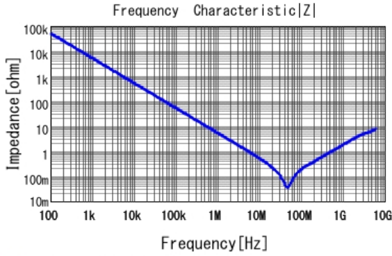
GCM155R71H333KE02 |Z| DCOV, 25degC
