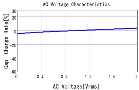
GCM155R71H333KE02 C-AC Voltage capchange, DCOV, 25.0d
