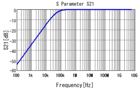
■ GCM155R71H333KE02 S21 DC0V, 25degC
