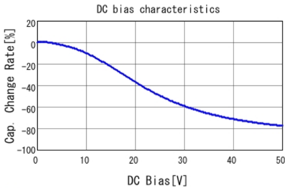
GCM155R71H333KE02 C-DC bias capchange, 25.0degC, AC1.
