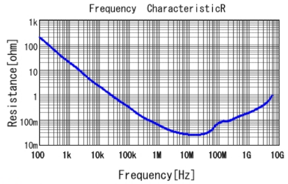
■ GCM155R71H473KE02 R DC0V, 25degC
