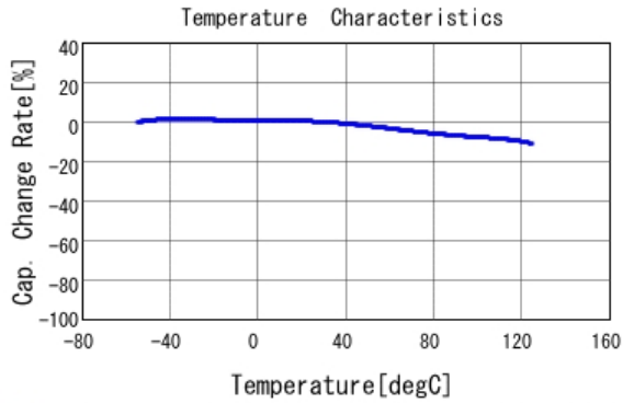
■ GCM155R71H473KE02 C-Temp. capchange, DC0.0V, AC1.0Vrm
