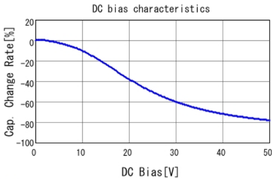
■ GCM155R71H473KE02 C-DC bias capchange, 25.0degC, AC1.
