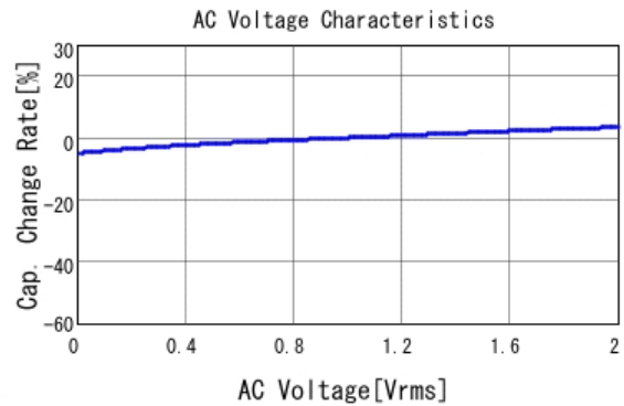
■ GCM155R71H473KE02 C-AC Voltage capchange, DC0V, 25.0d
