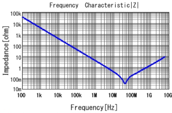
■ GCM155R71H473KE02 |Z| DC0V, 25degC
