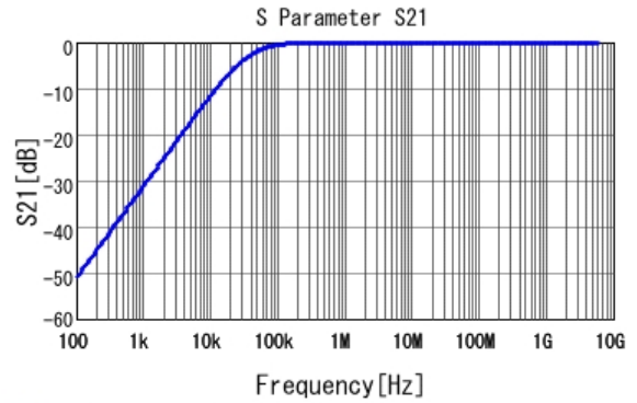
■ GCM155R71H473KE02 S21 DC0V, 25degC
