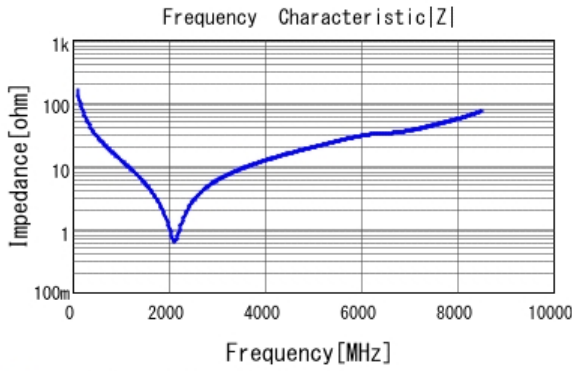
■ GCM1885C1H100JA16 |Z| DCOV, 25degC
