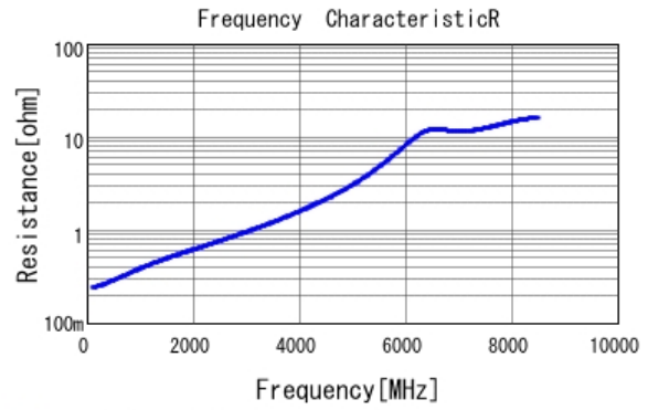
■ GCM1885C1H100JA16 R DCOV, 25degC
