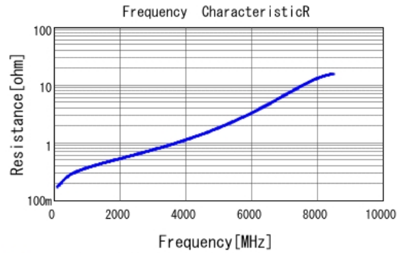
GCM1885C1H120JA16 R DCOV, 25degC
