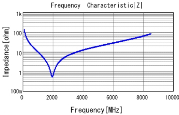
GCM1885C1H120JA16 |Z| DCOV, 25degC
