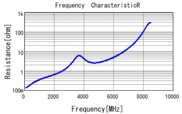
■ GCM1885C1H180JA16 R DCOV, 25degC
