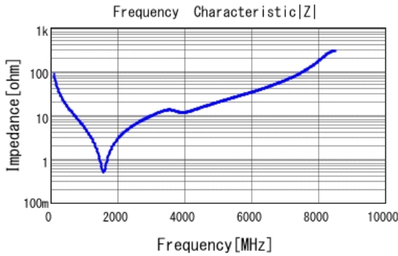
■ GCM1885C1H180JA16 |Z| DCOV, 25degC
