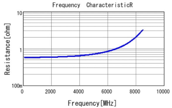
■ GCM1885C1H1R0CA16 R DCOV, 25degC
