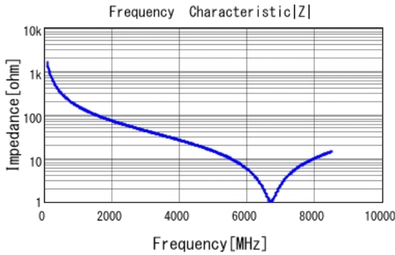
■ GCM1885C1H1R0CA16 |Z| DCOV, 25degC
