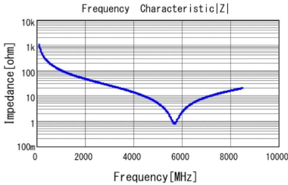
■ GCM1885C1H1R5CA16 |Z| DCOV, 25degC
