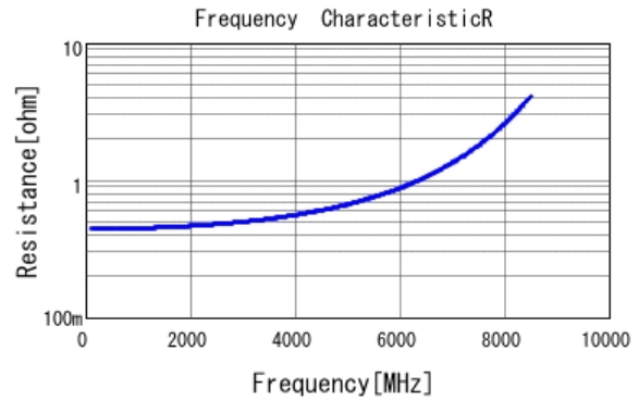
■ GCM1885C1H1R5CA16 R DCOV, 25degC
