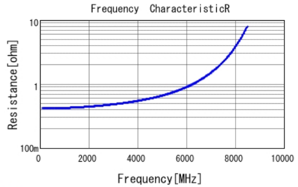
■ GCM1885C1H1R8BA16 R DCOV, 25degC
