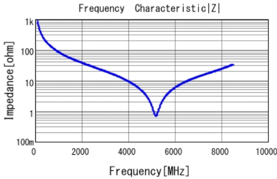
■ GCM1885C1H1R8BA16 |Z| DCOV, 25degC
