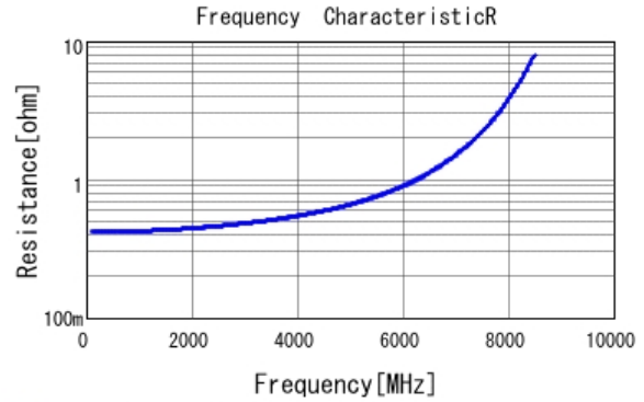
■ GCM1885C1H1R8CA16 R DCOV, 25degC
