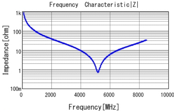
■ GCM1885C1H1R8CA16 |Z| DCOV, 25degC
