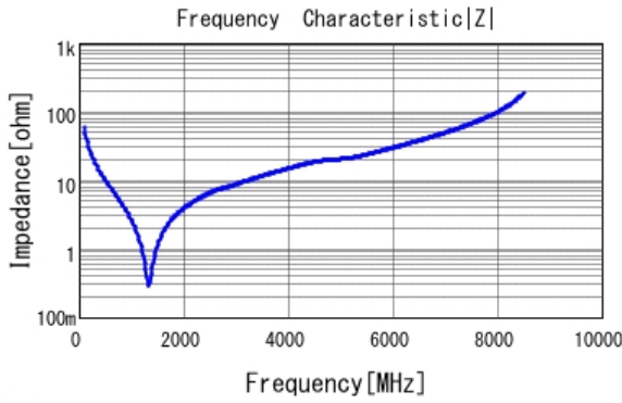
■ GCM1885C1H270JA16 |Z| DCOV, 25degC
