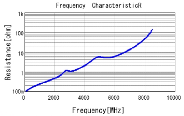
■ GCM1885C1H270JA16 R DCOV, 25degC
