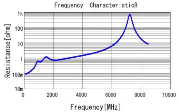
■ GCM1885C1H271JA16 R DCOV, 25degC
