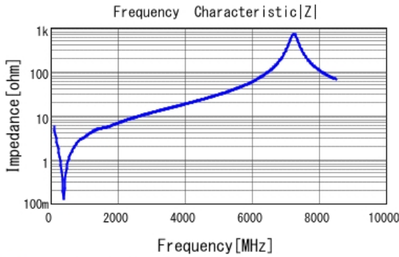
■ GCM1885C1H271JA16 |Z| DCOV, 25degC
