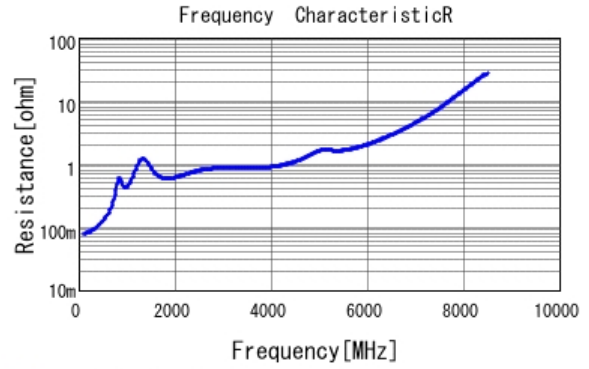
■ GCM1885C1H331JA16 R DCOV, 25degC
