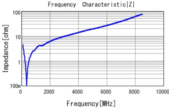
■ GCM1885C1H331JA16 |Z| DCOV, 25degC
