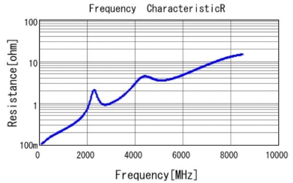
■ GCM1885C1H390JA16 R DCOV, 25degC
