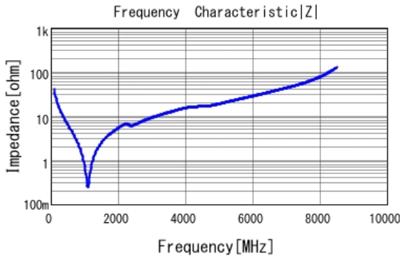
■ GCM1885C1H390JA16 |Z| DCOV, 25degC
