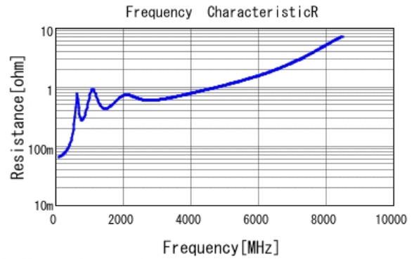
■ GCM1885C1H471JA16 R DCOV, 25degC
