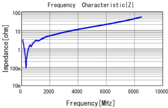
■ GCM1885C1H471JA16 |Z| DCOV, 25degC
