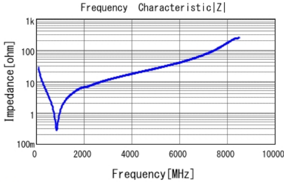
■ GCM1885C1H560JA16 |Z| DCOV, 25degC
