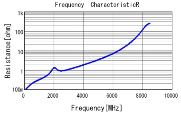
■ GCM1885C1H560JA16 R DCOV, 25degC
