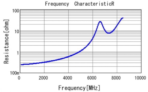
■ GCM1885C1H5R0CA16 R DCOV, 25degC
