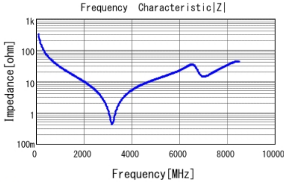
■ GCM1885C1H5R0CA16 |Z| DCOV, 25degC
